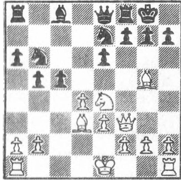
232 After 14...Nxe7
